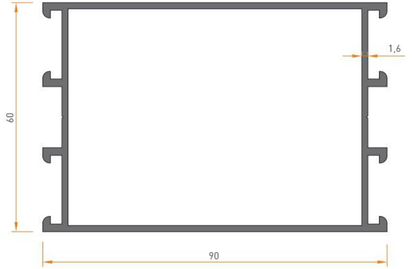
1984 GENİŞ KASA 1.475 kg/mt
