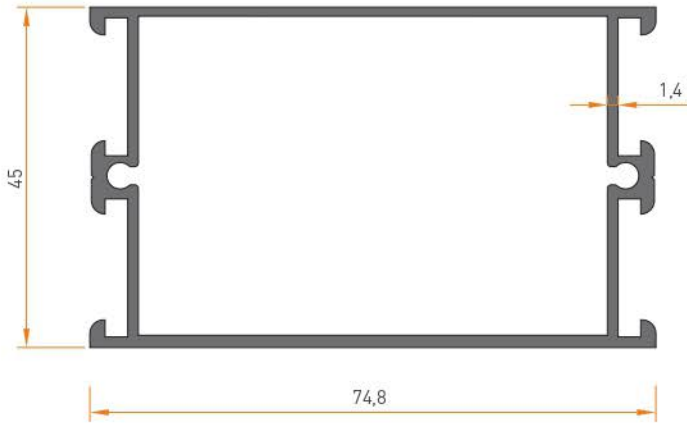
2017 GENİŞ KAYIT 1.080 kg/mt
