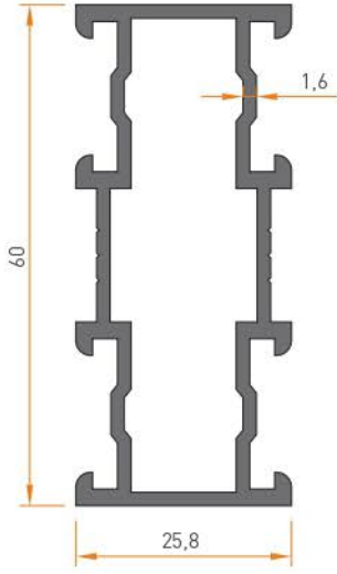
1977 DAR KASA 0.930 kg/mt
