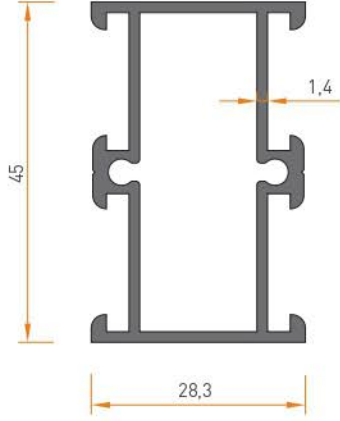
2014 DAR KAYIT 0.695 kg/mt
